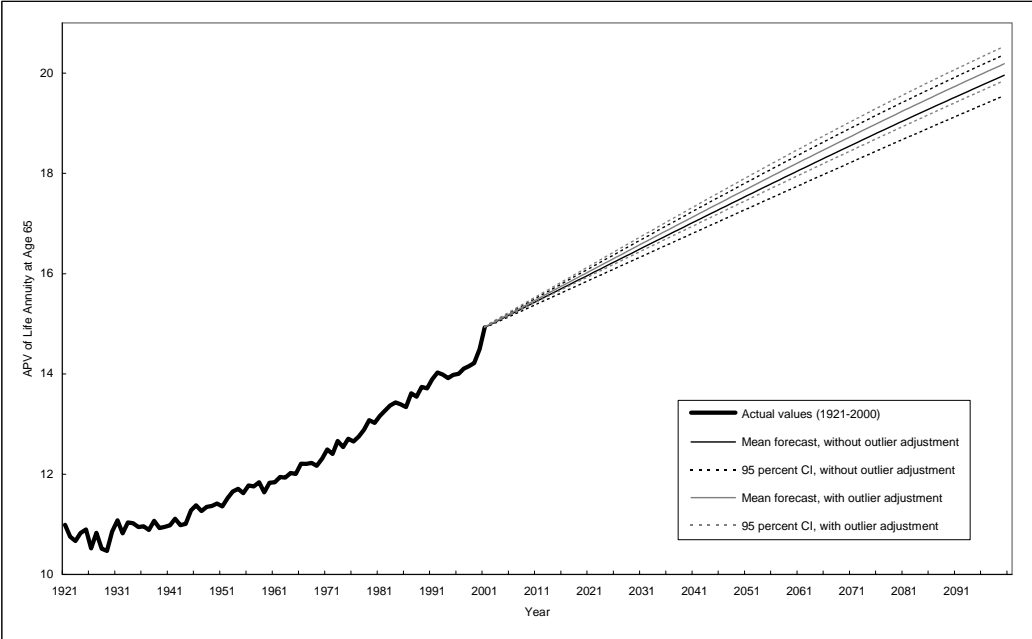
Figure 10 Mean Forecast and 95 Percent Pointwise Confidence Interval for the Actuarial Present Value of Life Annuity at Age 65, i = 2.5 percent, Canada
