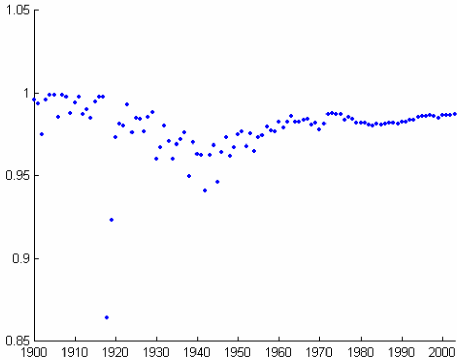
Figure 2: Correlation coefficients between the age-specific death rates per 100,000 by all causes and that by Influenza and Pneumonia, each year from 1900-2003
