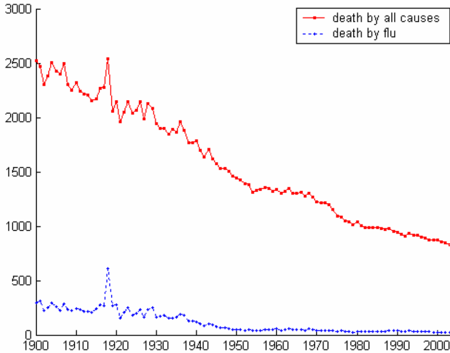
Figure 1: US age-adjusted death rate per 100,000 by all causes and by influenza and Pneumonia, from 1900 to 2003.
