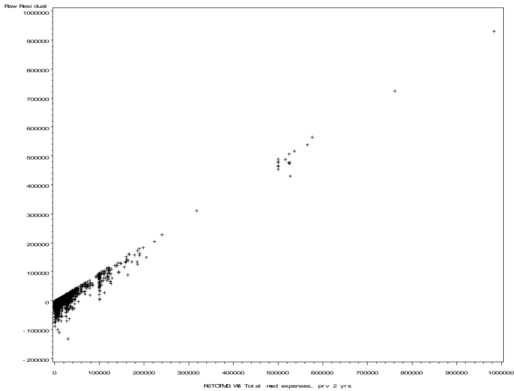
Fig. 4: Dollar-scale Residuals versus Actual Values for Part II ECM Poisson Model
