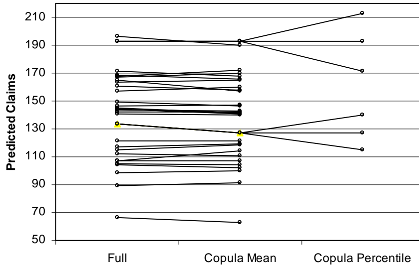
Figure 6. Distributions of copula credibility predictor
