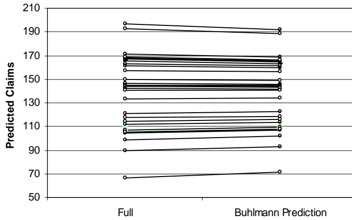
Figure 4. Shrinkage Effect of Bühlmann Credibility
