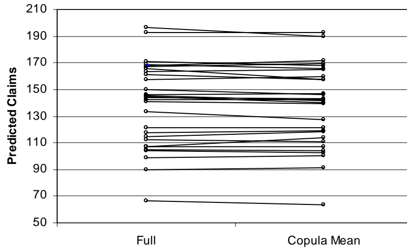
Figure 5. Shrinkage Effect of Copula Credibility Predictors
