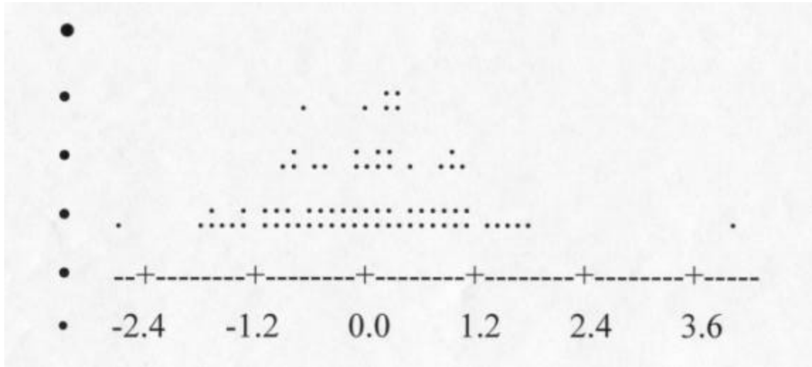
CHART 3 DOTPLOT OF STANDARDIZED RESIDUALS
