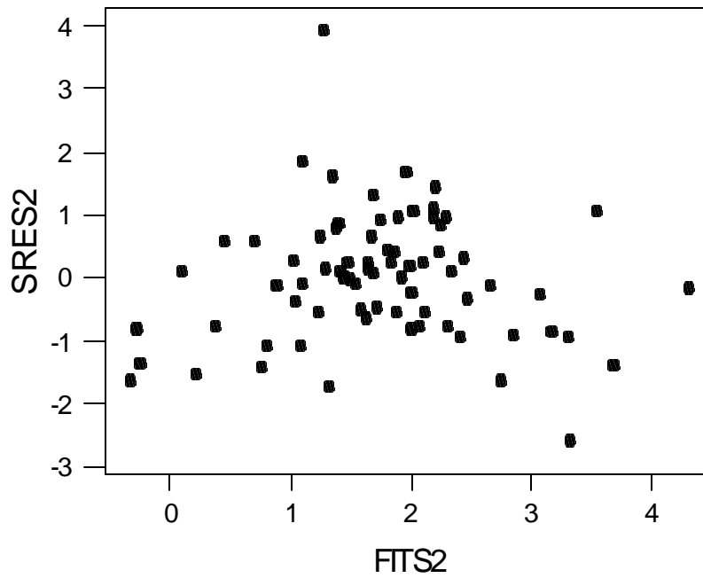
CHART 4 SCATTER PLOT OF THE STANDARDIZED RESIDUALS VERSUS THE FITTED VALUES
