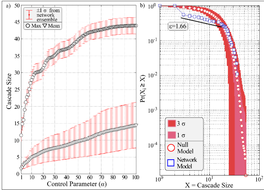
Figure 4: a) Maximum (circle) and mean (triangle) cascade size (y-axis) noted under each \alpha value, \alpha \in [1,100] . Error bars indicate one standard deviation across the ensemble of 1,000 networks; b) Cumulative probability distribution of cascade size, averaged across all \alpha . Results are for the cascade model (circle) and for a null model (square). One and three standard deviations are also shown for the latter.
