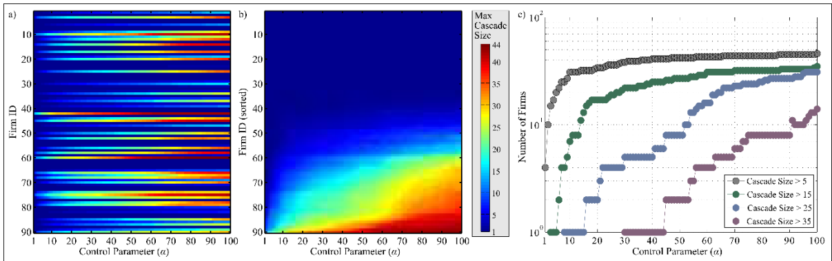
Figure 3: a) Cascade size (color) induced by the failure of firm i (y-axis) across the entire range of the control parameter \alpha , \alpha \in [1,100] (x-axis); b) same as a) though firms are now sorted in an ascending manner, based on the cascade size that their failure can induce under each \alpha value; c) number of firms (y-axis) capable of inducing a failure cascade greater than a given size (marker) under a given \alpha value (x-axis).
