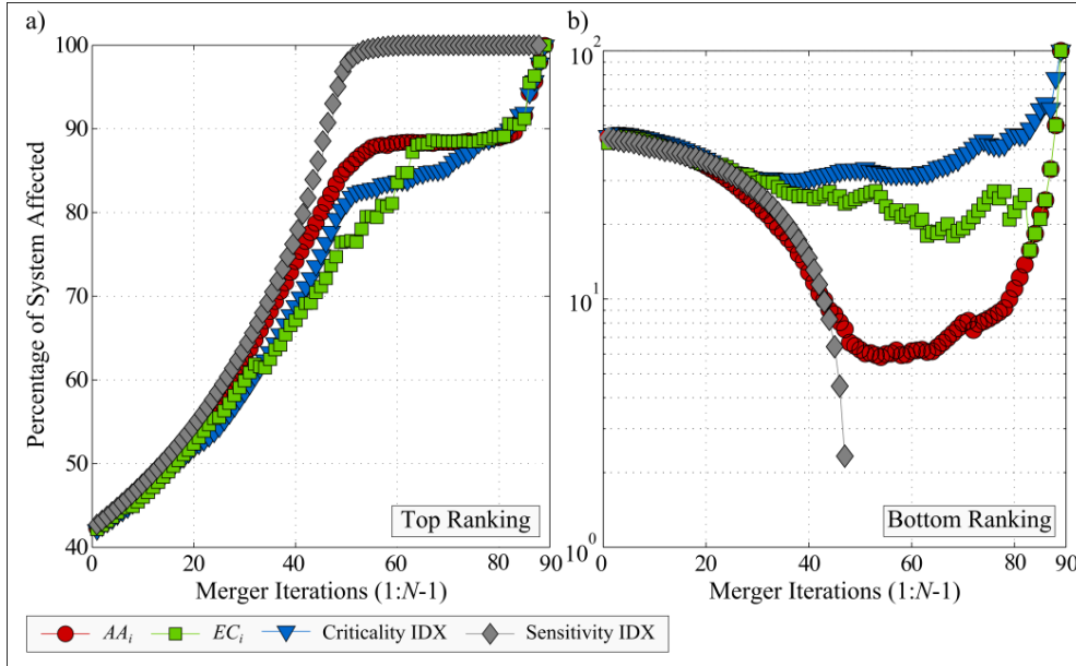
Figure 6: Robustness of the system as firms are iteratively merged, measured as the percentage of firms affected by the maximum failure cascade noted under failing each firm i , i \in N ; in a) the two highest-ranking firms are merged; in b) the two lowest-ranking firms are merged; note the logarithmic nature of the y-axis. Information used to enable this ranking is based on their Criticality IDX (triangle), Sensitivity IDX (diamond), AA_i (circle) or EC_i (square). Note that results are averaged across \alpha .
