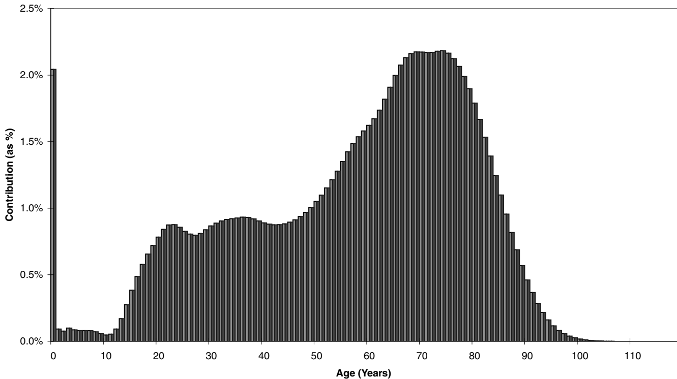
CONTRIBUTION BY YEAR OF AGE (AS %) TO SEX DIFFERENTIAL IN LIFE EXPECTANCY AT BIRTH IN 1990
