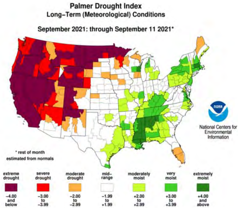
Figure 2.3.3.1 EXAMPLE OF THE PALMER DROUGHT INDEX
