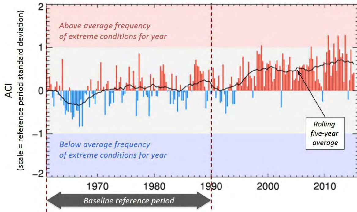
Figure 2.6.1 THE ACI FOR ALL OF NORTH AMERICA, ALONG WITH A FIVE-YEAR MOVING AVERAGE SHOWN IN BLACK.
