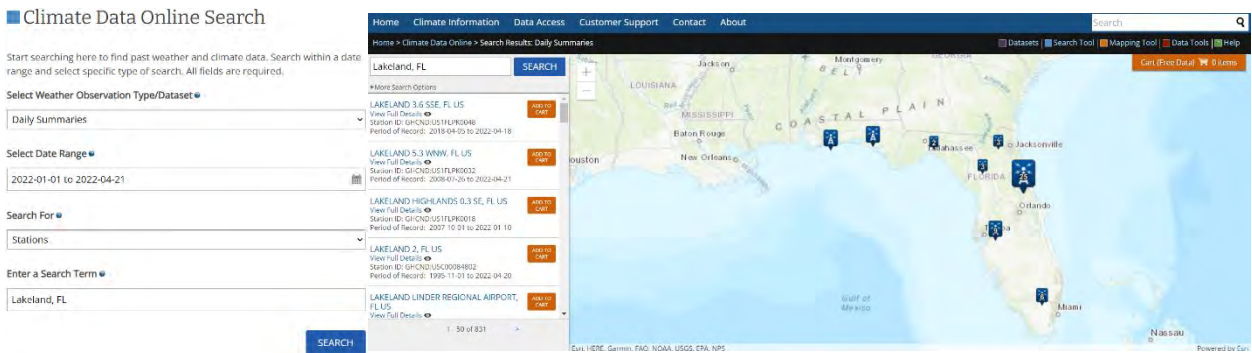
Figure 2.2.1 EXAMPLE OF THE CDO SEARCH TOOL , WITH THE FOUR MAIN CATEGORIES SHOWN ON THE LEFT AND THE ABILITY TO SELECT STATIONS USING THE MAP TOOL ON THE RIGHT. EXAMPLE DATA AVAILABLE TO DOWNLOAD.
